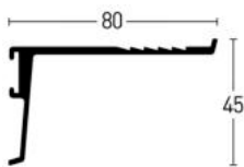
Profil 254 | Profile 254 Designboard
